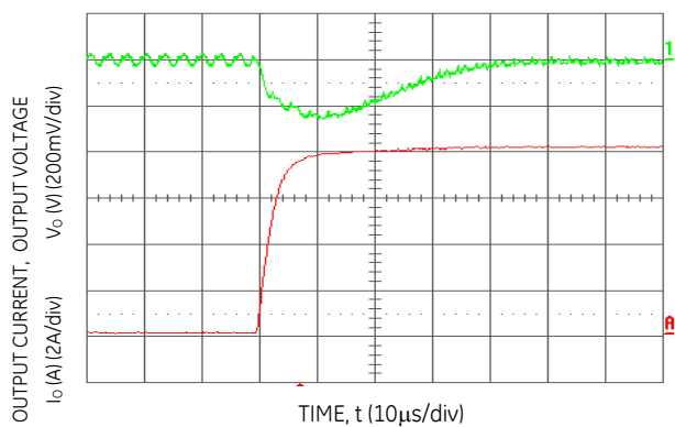
Figure 12. Transient Response to Dynamic Load Change from 50% to 100% of full load (Vo = 3.3Vdc, Cext = 2x150 µF Polymer Capacitors).
