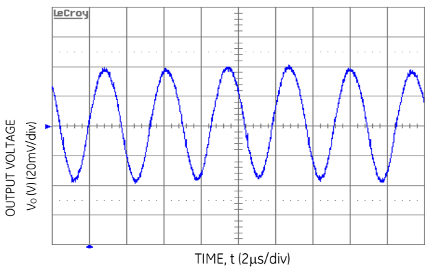
Figure 9. Typical Output Ripple and Noise (Vin = 12V dc, Vo = 3.3Vdc, Io=16A).
