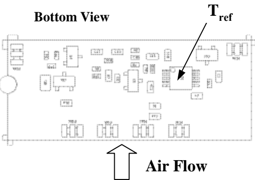
Figure 34. T ref Temperature measurement location.
