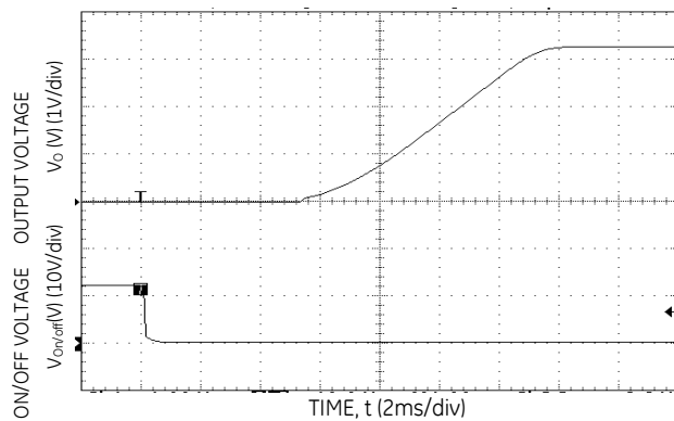
Figure 15. Typical Start-Up Using Remote On/Off with Low-ESR external capacitors (7x150uF Polymer) ( V_{in} = 12.0\text{Vdc} , V_o = 3.3\text{Vdc} , I_o = 3\text{A} , C_o = 1050\mu\text{F} ).
