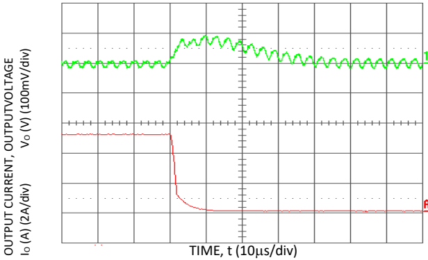
Figure 13. Transient Response to Dynamic Load Change from 100% of 50% full load (Vo = 5.0 Vdc, Cext = 2x150 μF Polymer Capacitors).
