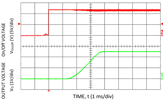
Figure 15. Typical Start-Up Using Remote On/Off with Low-ESR external capacitors (Co = 5000μF) (Vin = 12.0Vdc, Vo = 5.0Vdc, Io = 10.0A, Co = 1050μF).
