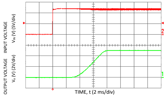
Figure 16. Typical Start-Up with application of Vin with low-ESR polymer capacitors at the output (7x150 μF) (Vin = 12Vdc, Vo = 5.0Vdc, Io = 10A, Co = 1050 μF).
