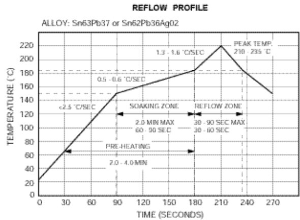
Figure 35. Reflow Profile.
