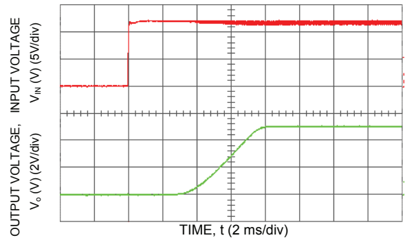
Figure 16. Typical Start-Up with application of V_{in} with low-ESR polymer capacitors at the output ( 7 \times 150\ \mu\text{F} ) ( V_{in} = 12\text{ Vdc} , V_o = 5.0\text{ Vdc} , I_o = 16\text{ A} , C_o = 1050\ \mu\text{F} ).
