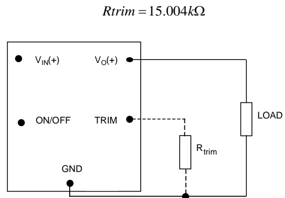
Figure 29. Circuit configuration to program output voltage using an external resistor.
