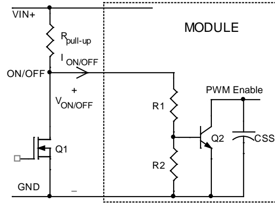
Figure 28. Circuit configuration for On/Off.
