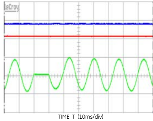
Figure 8. ½ cycle ride-through V IN 140 V AC
