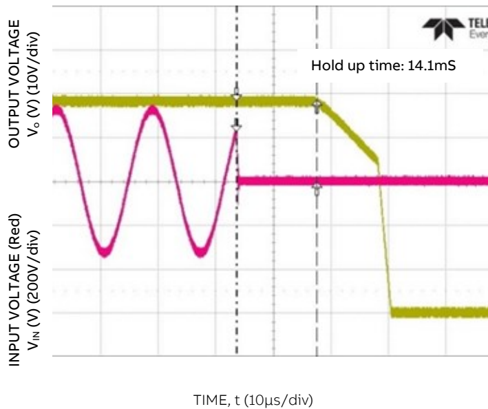
Figure 7. Typical Hold-up Waveforms ( V_{IN} = 230\text{V} , 100% Load)
