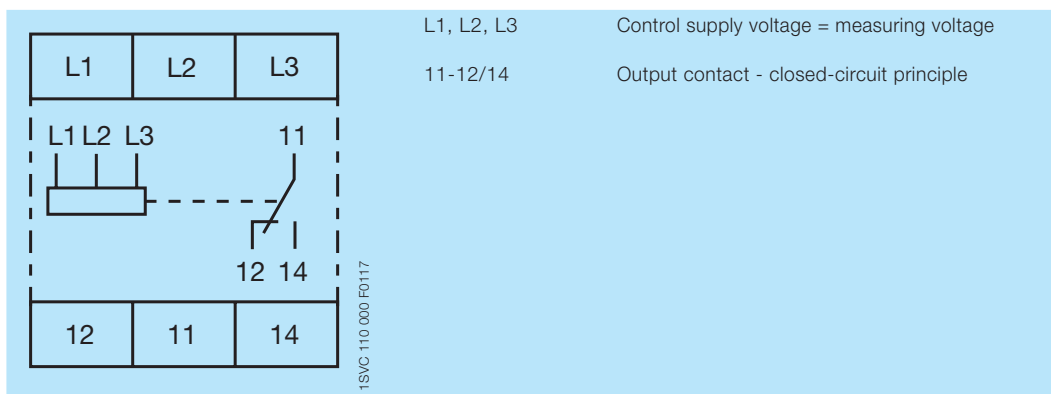
Connection diagram CM-PFD
