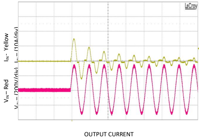
Figure 2. Inrush current V_{IN} = 230V_{AC} , 0^\circ phase angle
