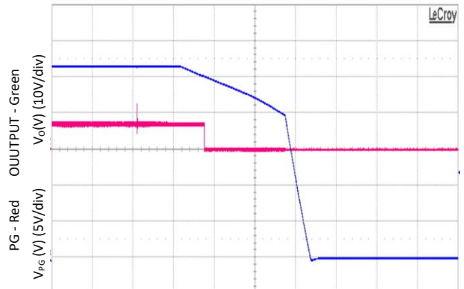
TIME, t (5ms/div)
