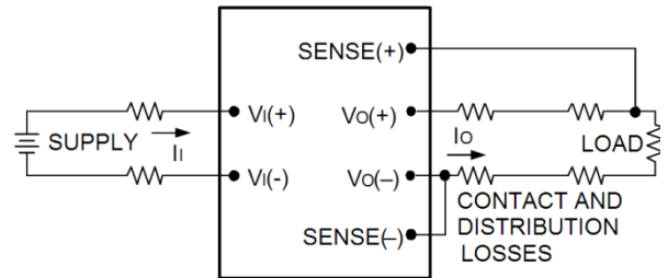
Figure 17. Circuit Configuration for remote sense.
