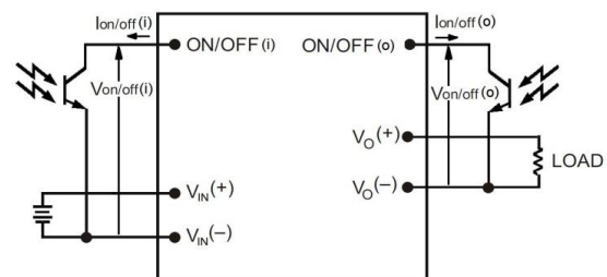
Figure 16. Remote On/Off Implementation.
