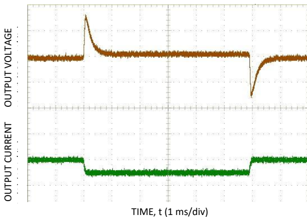
Figure 11. Typical Transient Response to Step Change in Load from 25% to 50% to 25% of Full Load at 48Vdc Input and C_o = 220\mu F Polymer, with -02 option.
