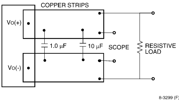
Figure 13. Input Reflected Ripple Current Test Setup.
