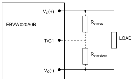
Figure 17. Circuit Configuration to Trim Output Voltage.
