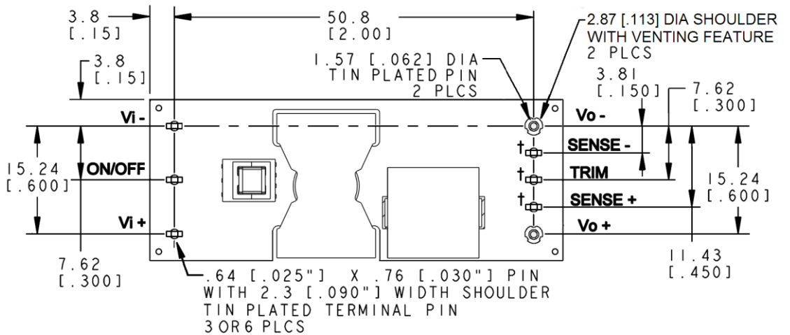
Bottom View
