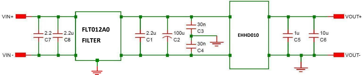
Figure 27. EMC Considerations
