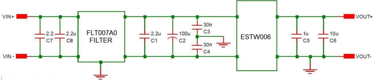
Figure 25. EMC Considerations.
