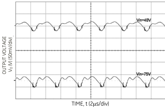
Figure 2. Typical output ripple and noise (Io = Io,max).
