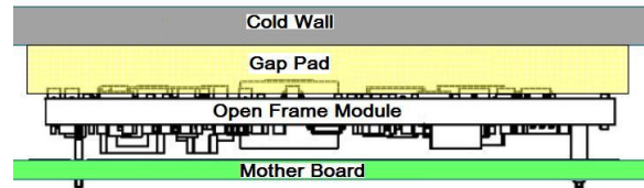
Figure 16. Cold Wall Mounting
