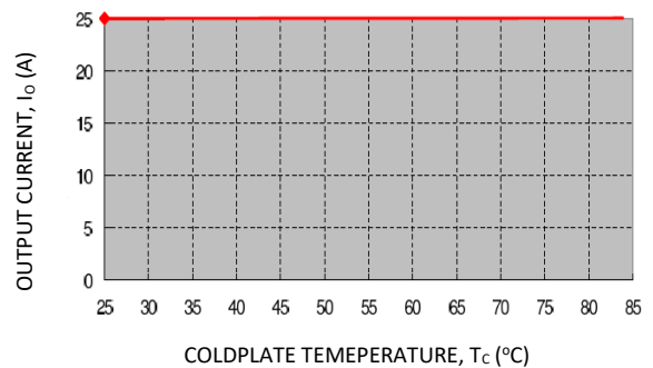
Figure 17. Derated Output Current versus Cold Wall Temperature with local ambient temperature around module at 85°C; V_{in}=48V .
