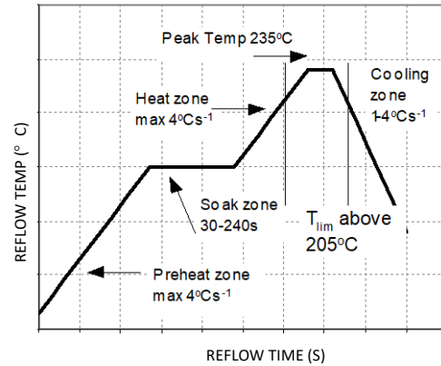
Figure 19. Reflow Profile for Tin/Lead (Sn/Pb) process.
