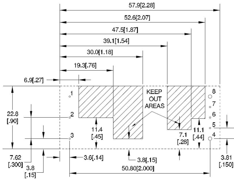
TH Recommended Pad Layout (Component Side View)
