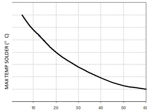
Figure 20. Time Limit Curve Above 205°C for Tin/Lead (Sn/Pb) process
