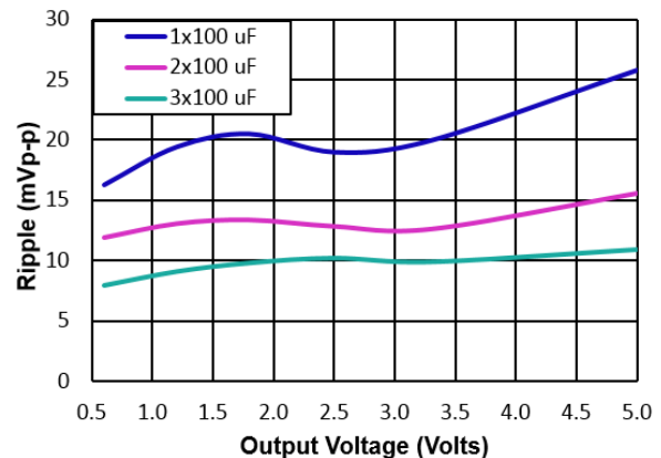
Figure 38. Output ripple voltage for various output voltages with external 1x100 \mu F, 2x100 \mu F, and 3x100 \mu F ceramic capacitors at the output (3A load). Input voltage is 12V.
