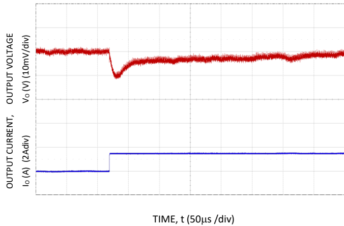
Figure 4. Transient Response to Dynamic Load Change from 50% to 100% at 12Vin, C out -2x330μF, 6x100μF, C tune -10nF, R tune -500
