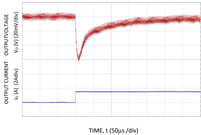
Figure 28. Transient Response to Dynamic Load Change from 50% to 100% at 12Vin, C_{out}=2\times 100\mu\text{F} , C_{tune}=1\text{nF} , R_{tune}=500
