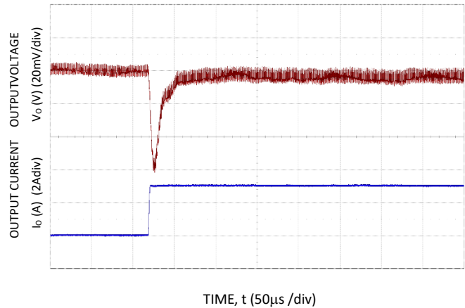
Figure 28. Transient Response to Dynamic Load Change from 50% to 100% at 12Vin, C_{out}=4\times 100\mu\text{F} , C_{tune}=2.2\text{nF} , R_{tune}=50\Omega
