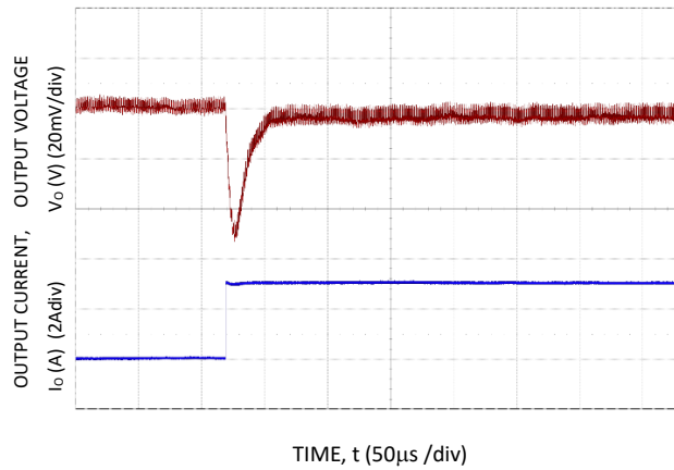
Figure 22. Transient Response to Dynamic Load Change from 50% to 100% at 12Vin, C_{out}=5 \times 100\mu\text{F} , C_{tune}=3.3\text{nF} , R_{tune}=500
