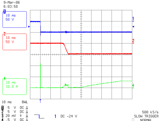
Figure 1. Inrush Current
