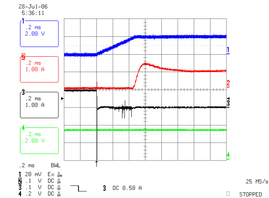
Figure 4. OR'ing Functionality when Feed B is shorted
