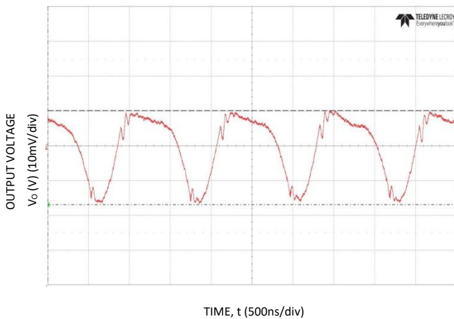
Figure 27. Typical output ripple and noise ( C_o=2x47\mu F ceramic, V_{IN} = 12V , I_o = I_{o,max} , 20MHz BW).
