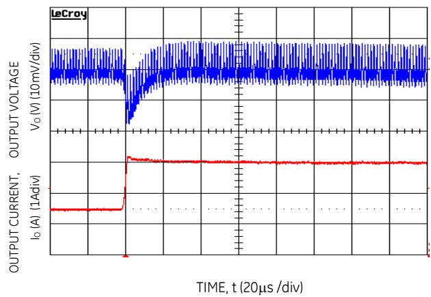
Figure 10. Transient Response to Dynamic Load Change from 50% to 100% at 12Vin, Cout-1x47uF+1x330uF, CTune-10nF & RTune-261
