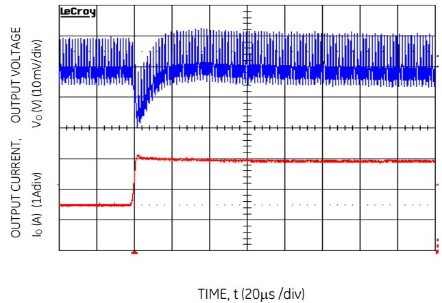
Figure 16. Transient Response to Dynamic Load Change from 50% to 100% at 12Vin, Cout-1x47uF+1x330uF, CTune-10nF & RTune-261
