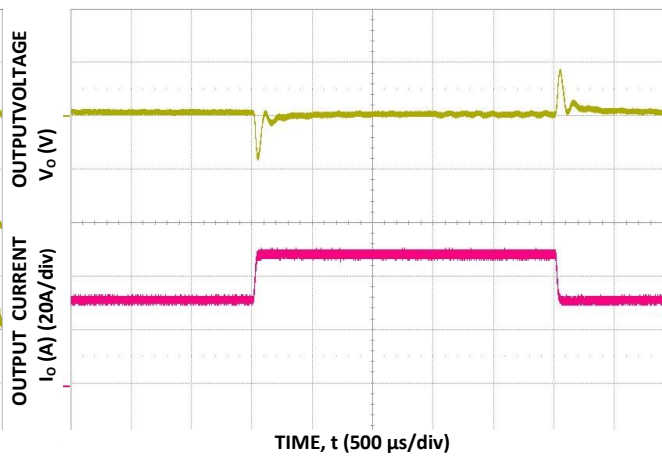
Figure 4. Typical Transient Response to 1.0A/ \mu s Step Change in Load from 50% to 75% to 50% of Full Load, C_o = 470\mu F and 50 V dc Input.
