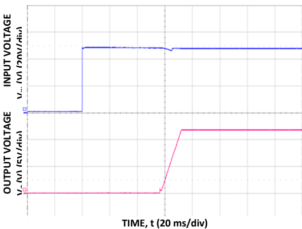
Figure 5. Typical Start-Up Using Vin with Remote On/Off enabled, negative logic version, without the -P option shown, I_o = I_{o,max} .
