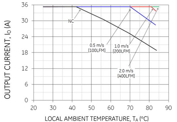
Figure 22. Output Current Derating for the Base plate QSVW035A0B-H with 1.0" heatsink in the Transverse Orientation; Airflow Direction from Vin(-) to Vin(+); Vin = 48V.
