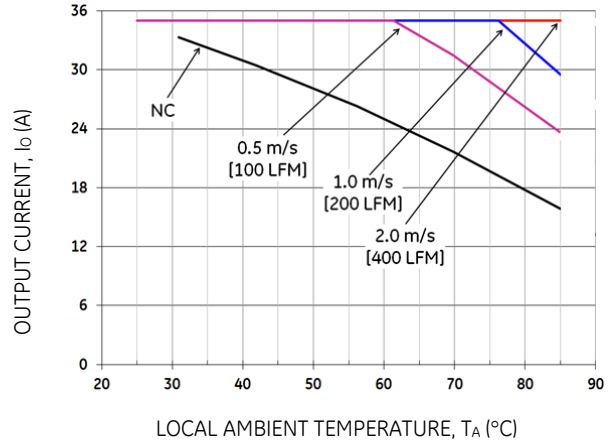
Figure 21. Output Current Derating for the Base plate QSVW035A0B-H with 0.5" heatsink in the Transverse Orientation; Airflow Direction from Vin(-) to Vin(+); Vin = 48V
