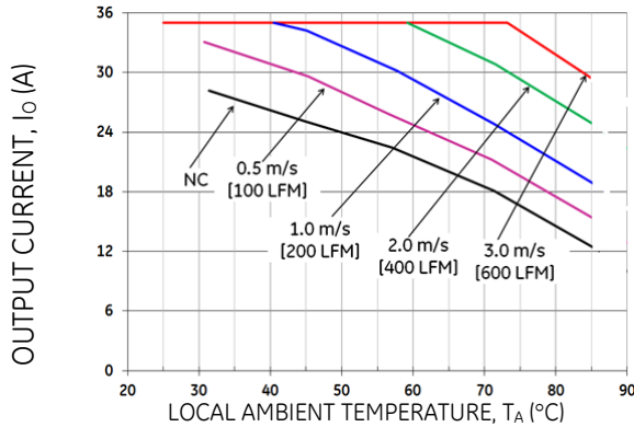
Figure 18. Output Current Derating for the Open Frame QSVW035A0B in the Transverse Orientation; Airflow Direction from Vin(-) to Vin(+); Vin = 48V.
