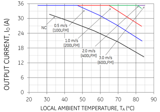
Figure 20. Output Current Derating for the Base plate QSVW035A0B-H with 0.25" heatsink in the Transverse Orientation; Airflow Direction from Vin(-) to Vin(+); Vin = 48V
