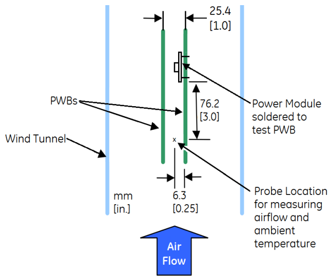
Figure 12. Thermal Test Setup .
