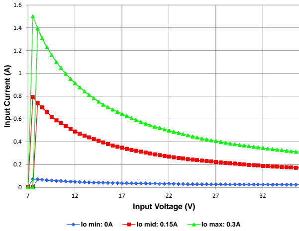
Figure 7. Input Current versus Input Voltage
