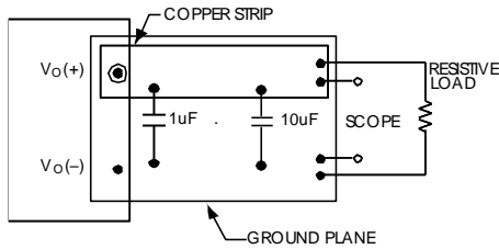
Figure 8. Input Reflected Ripple Current Test Setup.
