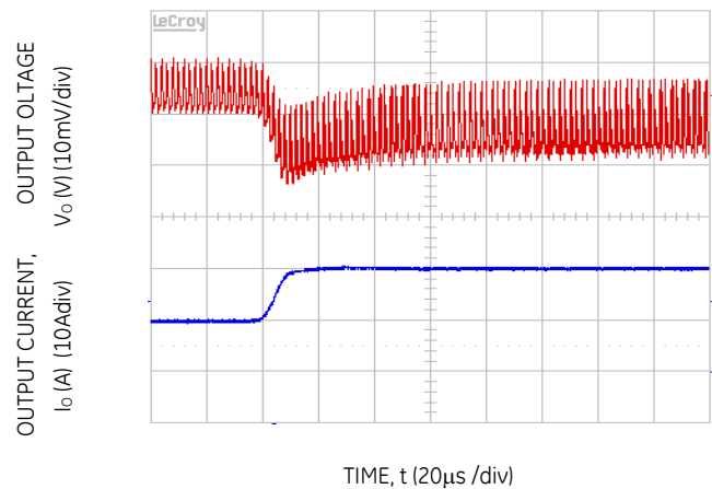
Figure 4. Transient Response to Dynamic Load Change from 50% to 100% at 12Vin, Cout= 1x47uF +11x330uF CTune=47nF, RTune=178 ohms
