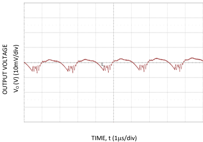
Figure 9. Typical output ripple ( C_o=8x47\mu F ceramic, V_{in} = 12V , I_o = I_{o,max} ).
