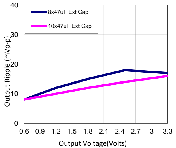
Figure 32. Output ripple voltage for various output voltages with external 8x47 μF or 10x47 μF ceramic capacitors at the output (35A load). Input voltage is 12V.
