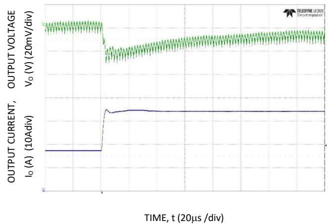
Figure 10. Transient Response to Dynamic Load Change from 50% to 100% at 12Vin, C_{out}=8x47\mu F+14x330\mu F , C_{Tune}=10nF , R_{Tune}=300\Omega
