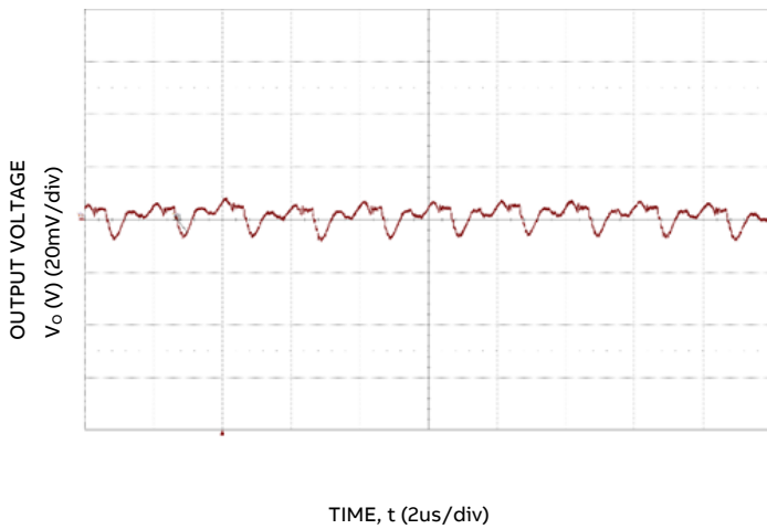
Figure 27. Typical output ripple and noise ( C_o = 4 \times 0.1\mu F + 12 \times 47\mu F + 2 \times 330\mu F polymer, V_{in} = 12V , I_o = I_{o,max} ).
