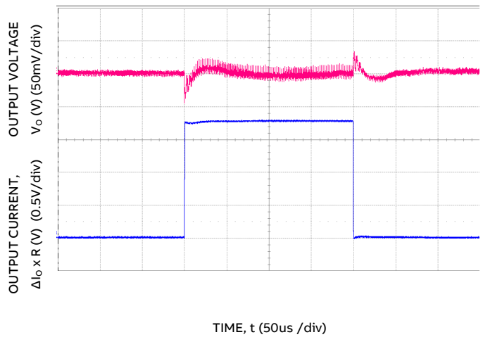
Figure 28. Transient Response to 100A/μs Dynamic Load Change from 25% to 75% at 12Vin ( C_o = 4 \times 0.1\mu F + 12 \times 47\mu F + 12 \times 1500\mu F , ASCR Gain = 256, ASCR Integrator = 128, ASCR Residual = 64). \Delta I_o = 1.772V / (0.2\Omega / 4) = 35.4A
