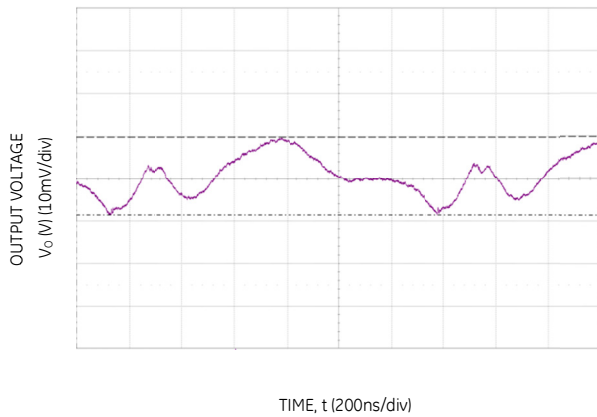
Figure 9. Typical output ripple and noise ( C_o=1x47\mu F ceramic, V_{IN} = 12V , I_o = I_{o,max} ).
