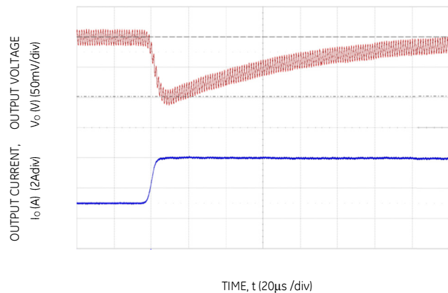
Figure 34. Transient Response to Dynamic Load Change from 50% to 100% at 12Vin, C_{out} = 3 \times 47 \mu F , C_{Tune} = 1500 pF & R_{Tune} = 300 \Omega
