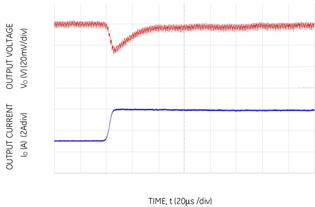
Figure 10. Transient Response to Dynamic Load Change from 50% to 100% at 12Vin, C_{out} = 3x47\mu F+1x330\mu F , C_{Tune} = 4700pF & R_{Tune} = 300\Omega
