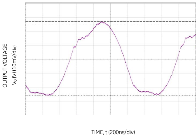
Figure 33. Typical output ripple and noise ( C_o=1 \times 47 \mu F ceramic, V_{IN} = 12V , I_o = I_{o,max} ).
