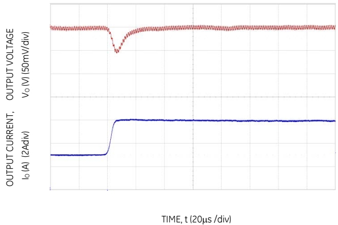
Figure 22. Transient Response to Dynamic Load Change from 50% to 100% at 12Vin, Cout = 4x47uF, CTune=2700pF & RTune=300Ω
