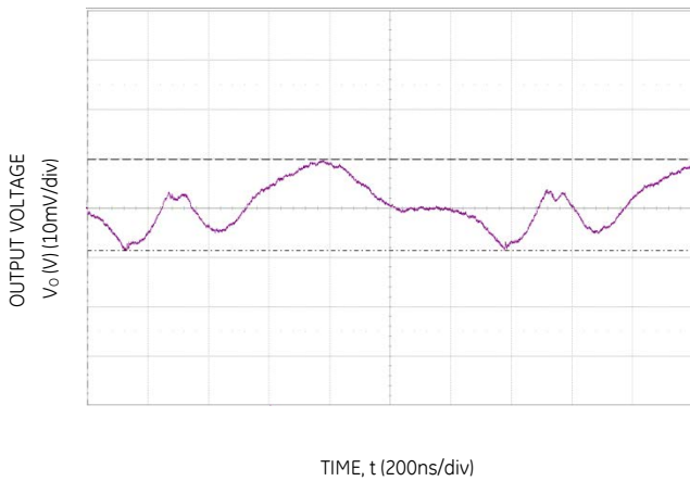
Figure 9. Typical output ripple and noise (C o =1x47μF ceramic, V IN = 12V, I o = I o,max ).
