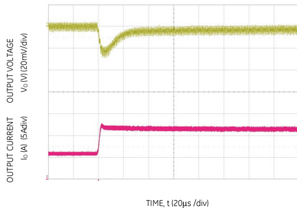
Figure 10. Transient Response to Dynamic Load Change from 50% to 100% at 12Vin, Cout = 3x47uF+3x330uF, CTune = 12nF & RTune = 220 ohms
