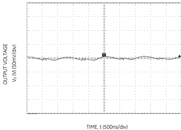
Figure 3. Typical output ripple and noise ( C_o=2 \times 47 \mu F ceramic, V_{IN} = 12V , I_o = I_{o,max} ).
