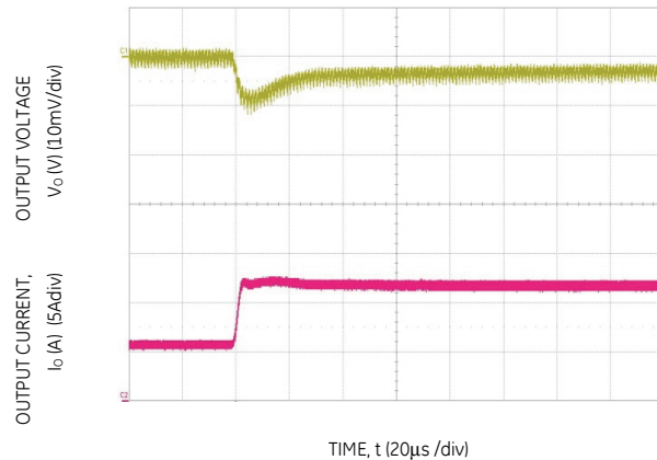
Figure 4. Transient Response to Dynamic Load Change from 50% to 100% at 12Vin, C_{out}=1 \times 47 \mu F + 11 \times 330 \mu F , C_{Tune}=47nF , R_{Tune}=180 \Omega
