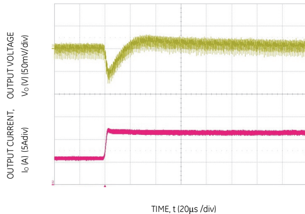
Figure 22. Transient Response to Dynamic Load Change from 50% to 100% at 12Vin, C_{out} = 2 \times 47 \mu F + 1 \times 330 \mu F , C_{Tune}=4700pF & R_{Tune}=240 \Omega
