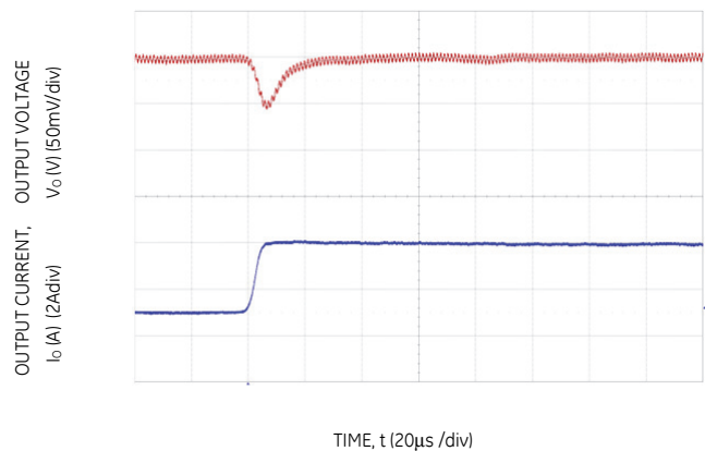
Figure 22. Transient Response to Dynamic Load Change from 50% to 100% at 12Vin, C_{out} = 4x47\mu F , C_{Tune}=2700pF & R_{Tune}=300\Omega
