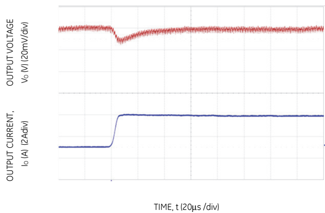
Figure 4. Transient Response to Dynamic Load Change from 50% to 100% at 12Vin, Cout=3x47uF+3x330uF, CTune=15nF, RTune=200Ω
