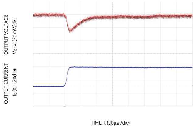
Figure 10. Transient Response to Dynamic Load Change from 50% to 100% at 12Vin, Cout = 3x47uF+1x330uF, CTune = 4700pF & RTune = 300Ω
