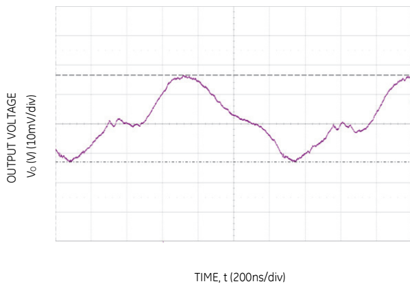
Figure 21. Typical output ripple and noise ( C_O=1x47\mu F ceramic, V_{IN} = 12V , I_o = I_{o,max} ).
