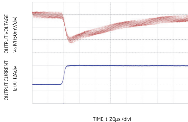
Figure 34. Transient Response to Dynamic Load Change from 50% to 100% at 12Vin, C_{out} = 3x47\mu F , C_{Tune}=1500pF & R_{Tune}=300\Omega
