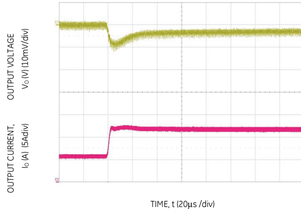
Figure 4. Transient Response to Dynamic Load Change from 50% to 100% at 12Vin, C out =1x47uF+11x330uF, CTune=47nF, RTune=180Ω
