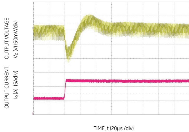
Figure 34. Transient Response to Dynamic Load Change from 50% to 100% at 12Vin, Cout = 1x47µF+1x330µF, CTune=2200pF & RTune=300Ω
