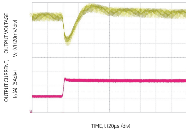
Figure 16. Transient Response to Dynamic Load Change from 50% to 100% at 12Vin, C out = 2x47µF+2x330µF, C Tune =5600pF & R Tune =220Ω
