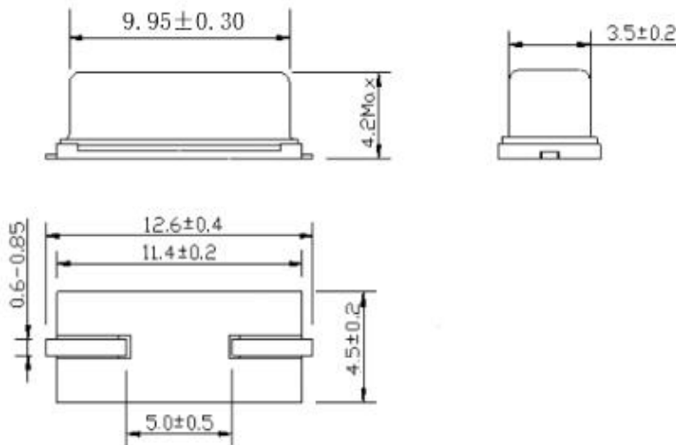
Dimensions(mm)
