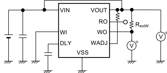
Figure 28 Test Circuit 10
