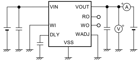
Figure 20 Test Circuit 2
