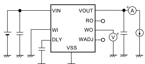
Figure 24 Test Circuit 6
