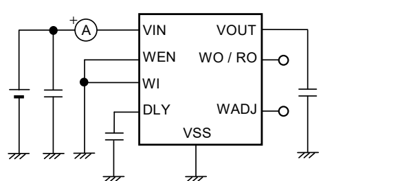
Figure 18 Test Circuit 10
