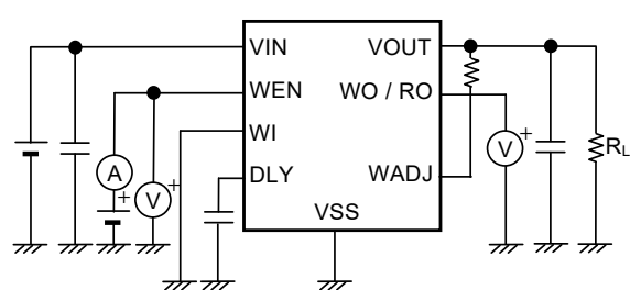
Figure 16 Test Circuit 8
