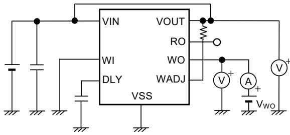
Figure 29 Test Circuit 11
