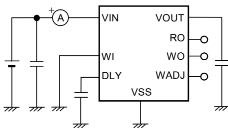
Figure 27 Test Circuit 9
