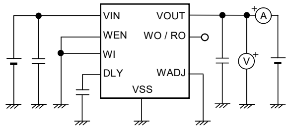
Figure 10 Test Circuit 2
