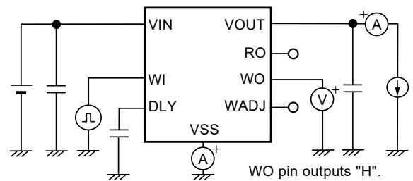
Figure 26 Test Circuit 8
