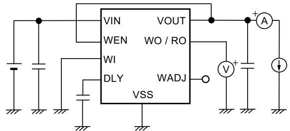
Figure 14 Test Circuit 6
