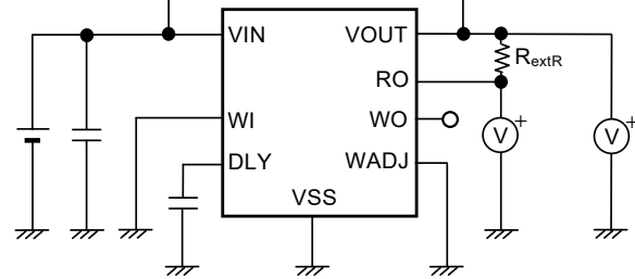
Figure 22 Test Circuit 4
