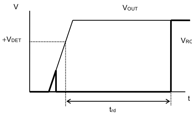
Figure 5 Release Delay Time
