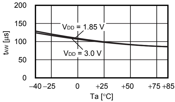
3.5 Awake mode time ( t_{AW} ) vs. Temperature ( T_a )
