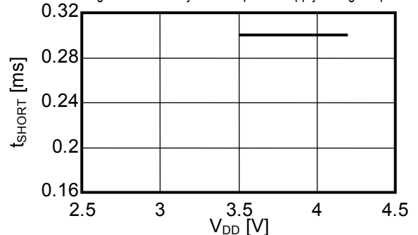
Load short-circuiting detection delay time vs. power supply voltage dependency
