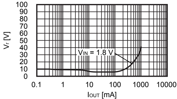
Condition 3 S-8366AABBA ( V_{OUT(S)} = 2.5\text{ V} )
