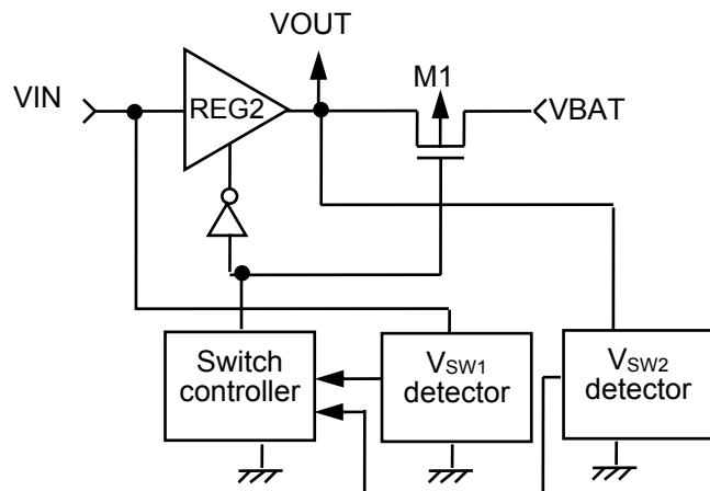
Figure 8 Switch Unit
