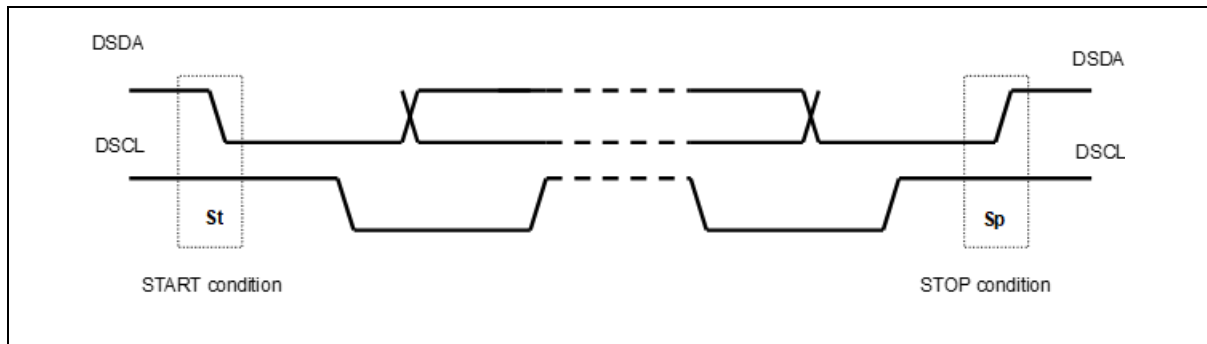
Figure 37. Start and Stop Condition
