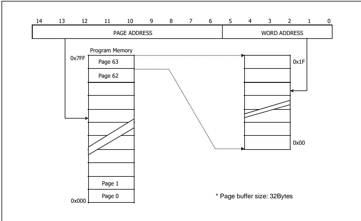
Figure 23. Address Configuration of Flash Memory
