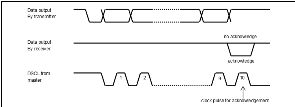
Figure 38. Acknowledge on Serial Bus
