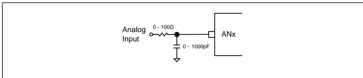
Figure 19. A/D Analog Input Pin with a Capacitor
