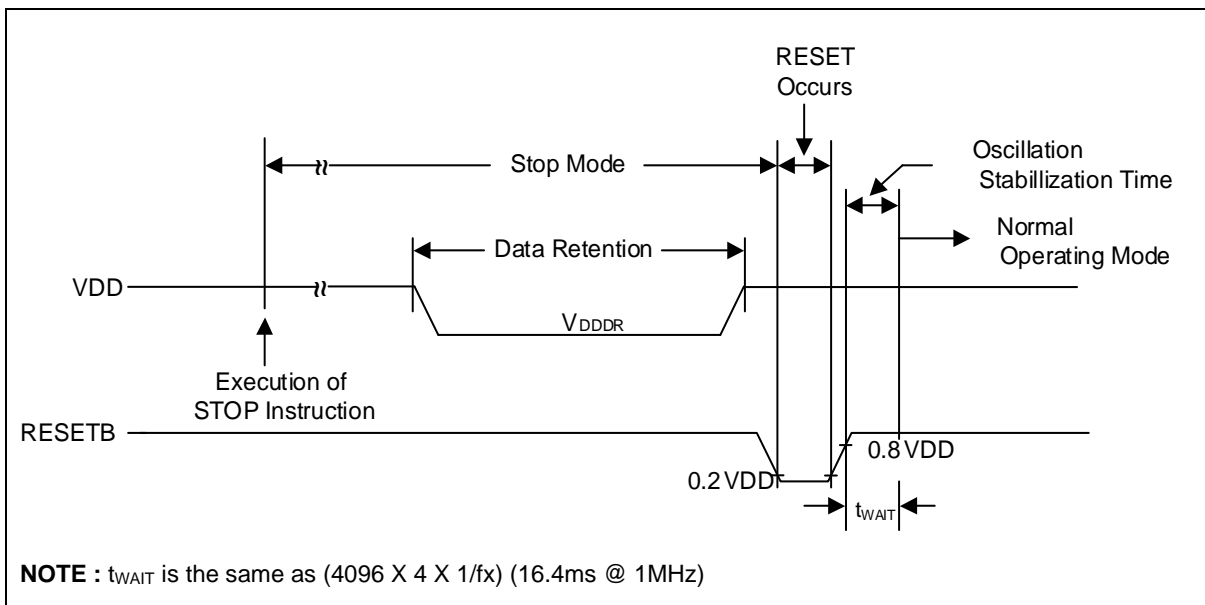
Figure 26. Stop Mode Release Timing when Initiated by RESETB
