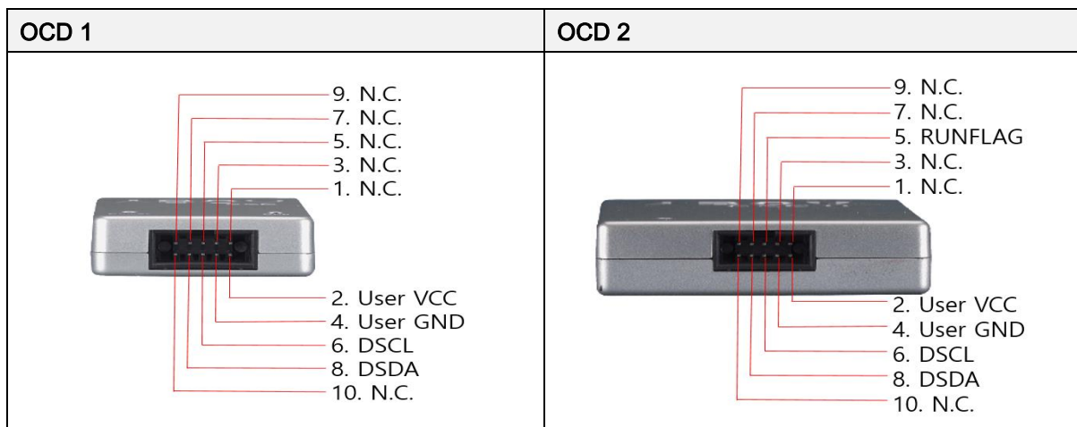
Figure 30. OCD 1 and OCD 2 Connector Pin Diagram
