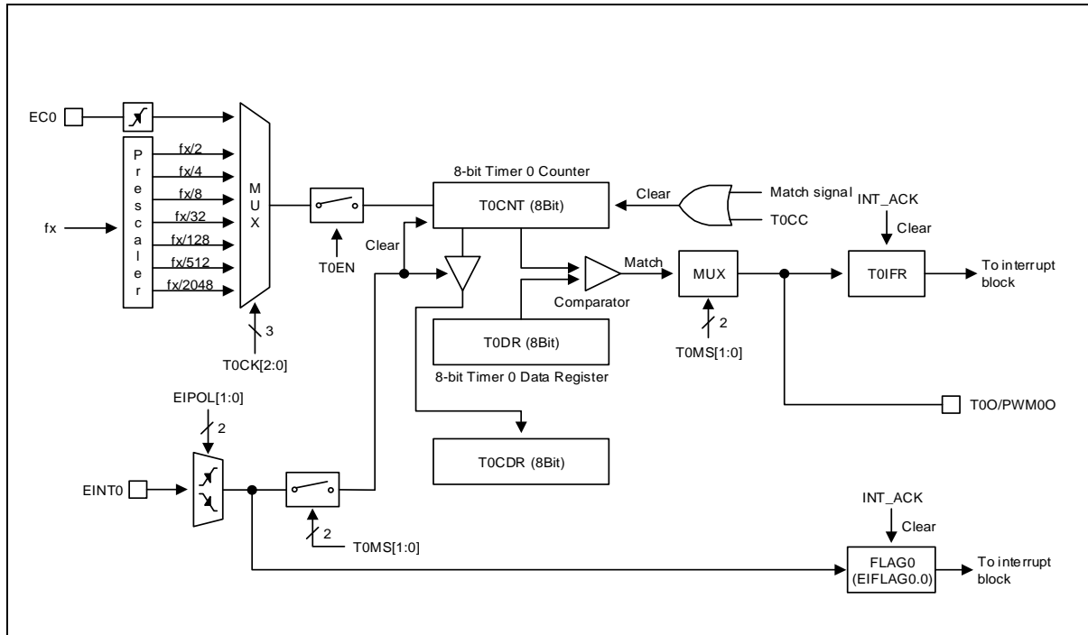
Figure 15. 8-bit Timer 0 Block Diagram
