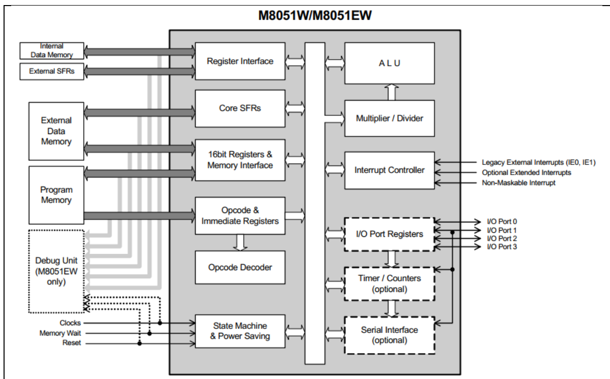
Figure 6 M8051EW Architecture
