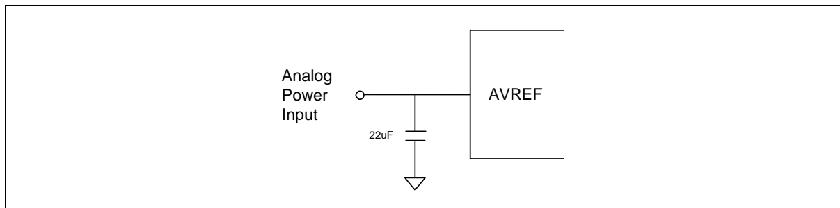
Figure 20. A/D Power (AVREF) Pin with a Capacitor
