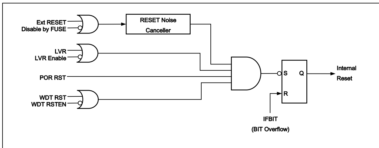
Figure 21. Reset Block Diagram
