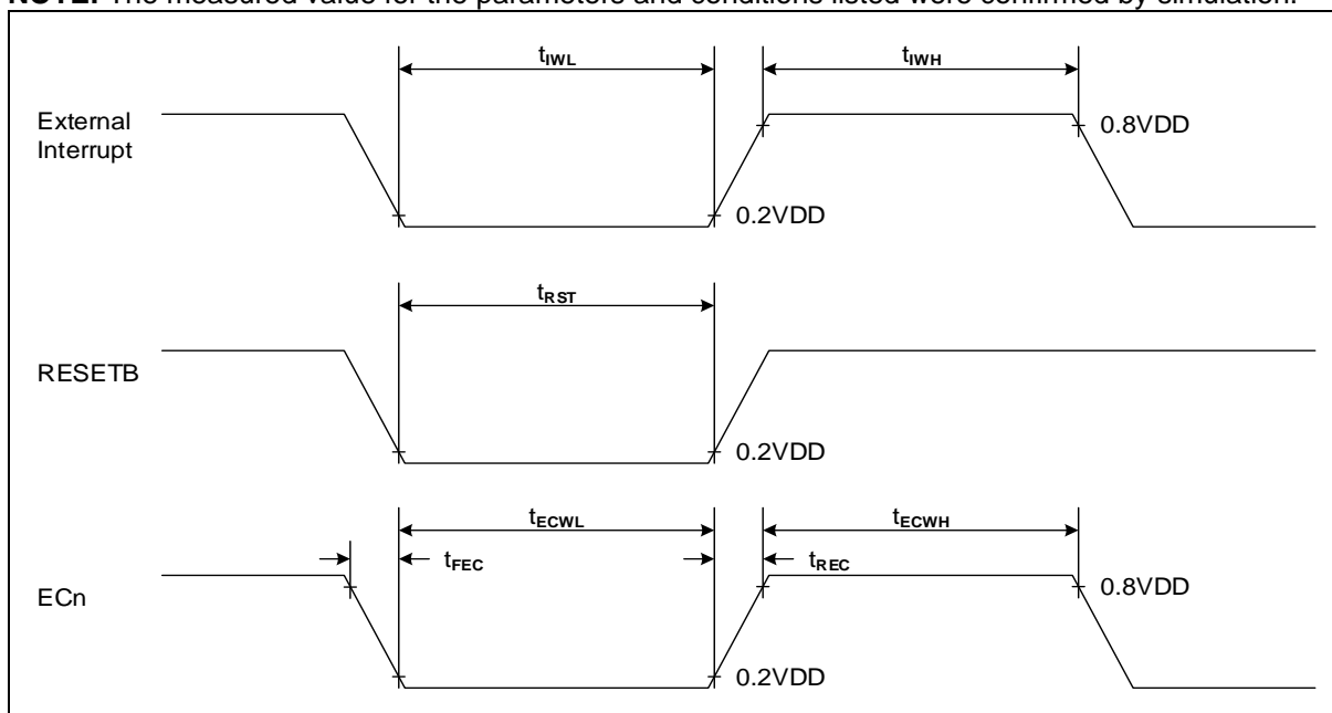
Figure 24. AC Timing
