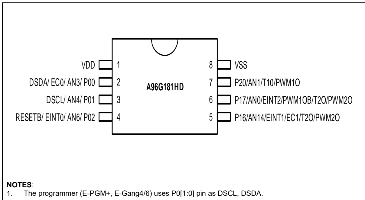
Figure 3. A96G181 8SOP pin assignment
