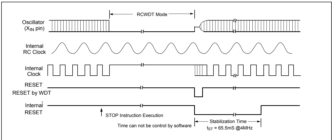
Figure 17-8 Internal RC-WDT Mode Releasing by Reset
