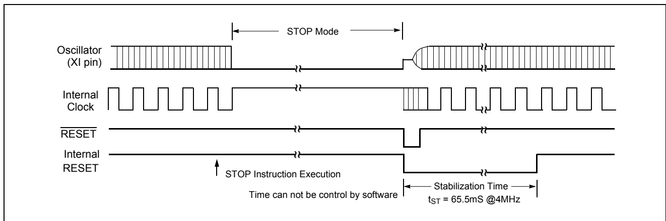
Figure 17-6 Timing of STOP Mode Release by Reset
