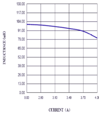
ASPI-1306T-101M
