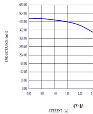
ASPI-1306T-471M
