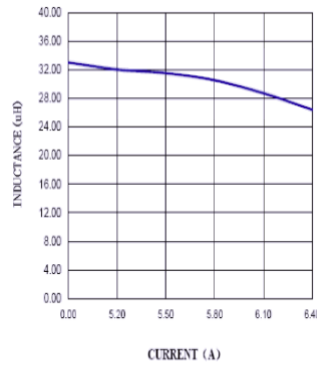
ASPI-1306T-330M
