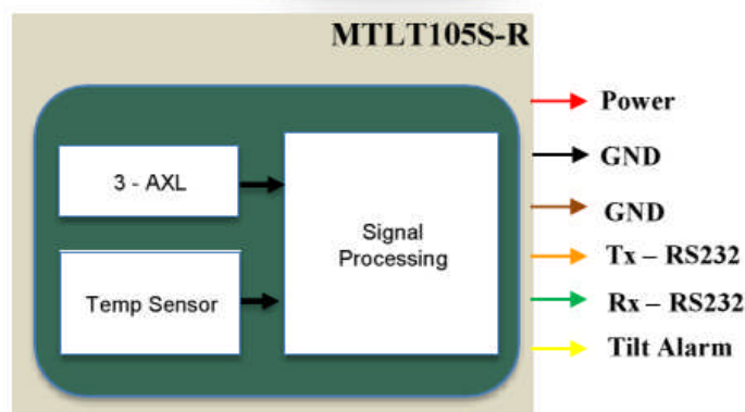
Platform Leveling
