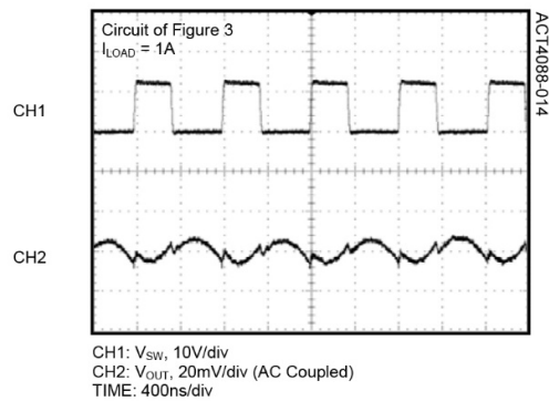
Figure 5: Circuit of Figure 3 ( I_{LOAD} = 1A )
