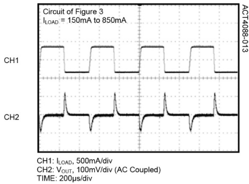
Figure 4: Circuit of Figure 3 ( I_{LOAD} = 150mA to 850mA )
