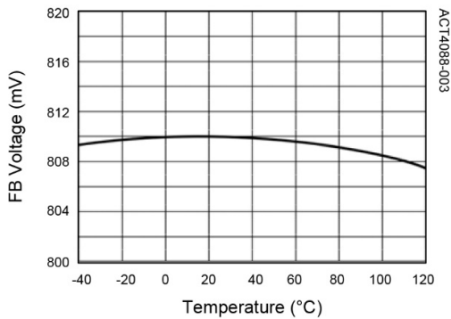
FB Voltage vs. Temperature
