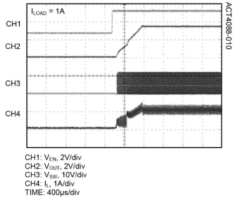
Start-up Waveforms
