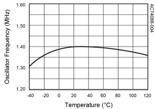
Oscillator Frequency vs. Temperature
