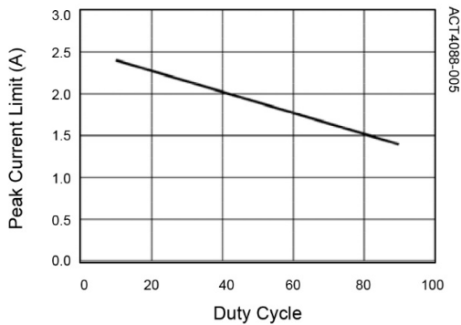
Peak Current Limit vs. Duty Cycle
