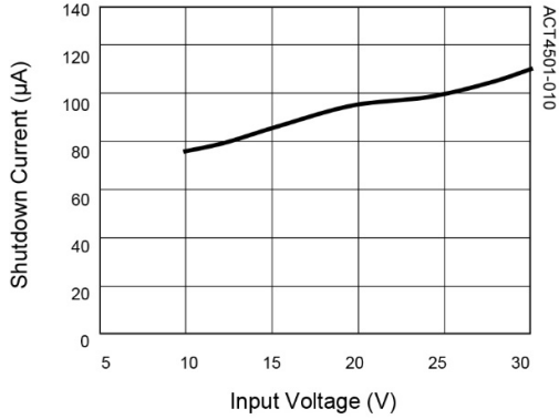
Shutdown Current vs. Input Voltage (EN pulled low)
