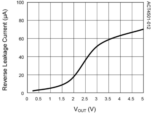
Reverse Leakage Current (V IN Floating)
