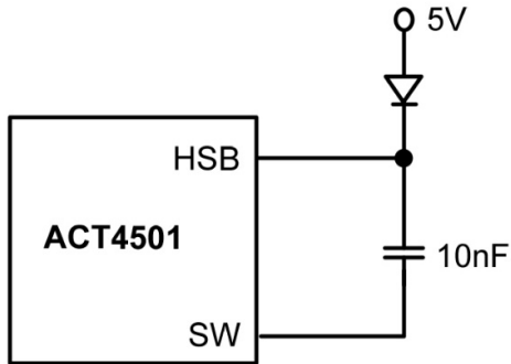
Figure 3: External High Voltage Bias Diode
