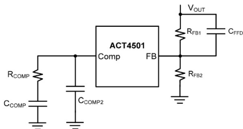
Figure 6: Frequency Compensation for High R FB1
