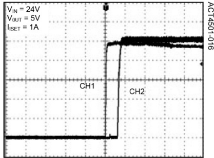
Start up with EN
