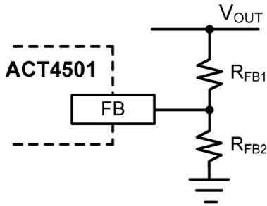
Figure 1: Output Voltage Setting
