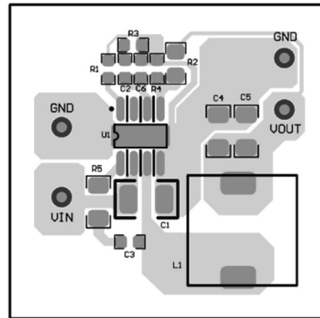
Figure 7: PCB Layout
