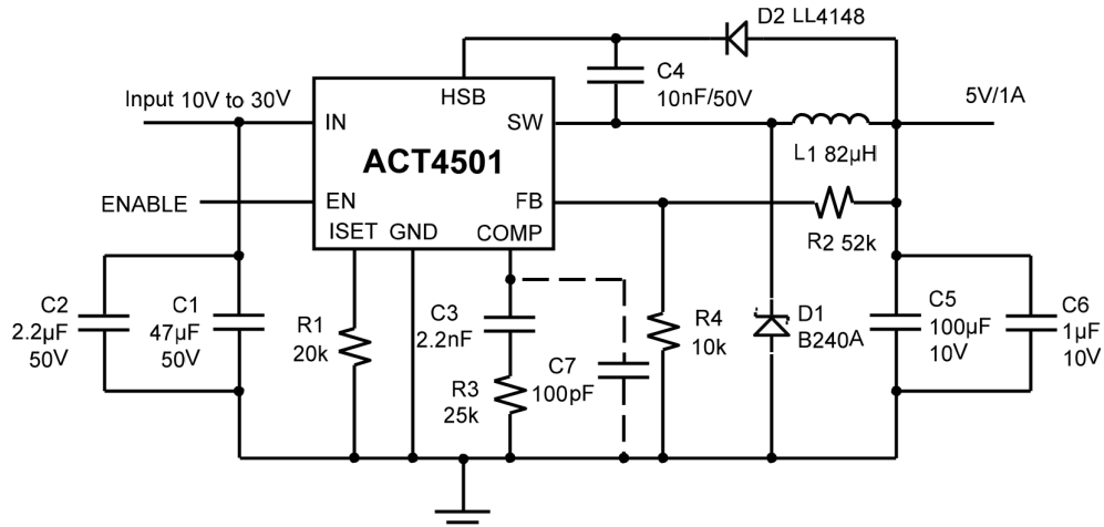
Figure 8: Typical Application Circuit for 5V/1A Car Charger
