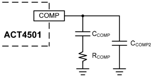
Figure 4: Stability Compensation
