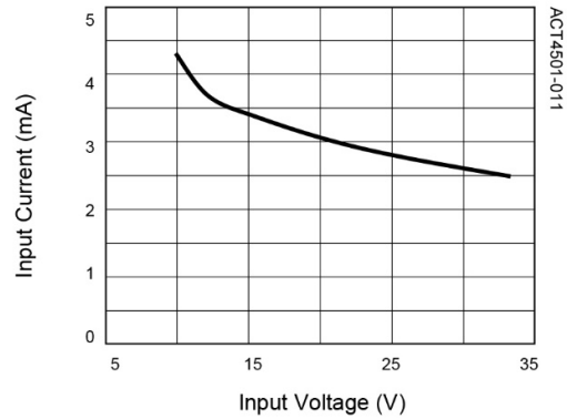
Standby Supply Current vs. Input Voltage
