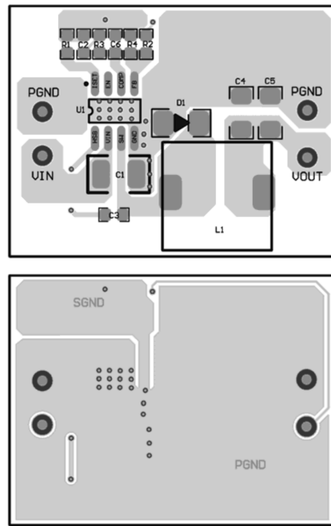
Figure 8: PCB Layout
