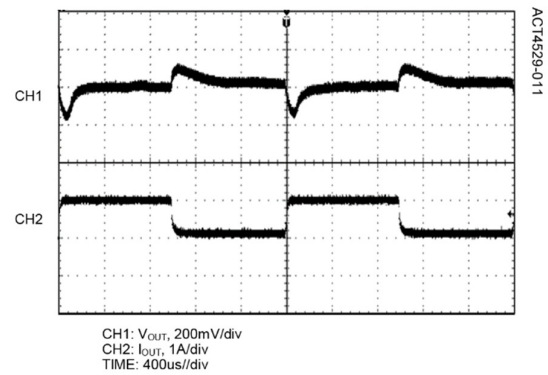
Load Transient (80mA-1A-80mA) V_{in}=12.6\text{V} , V_{out}=12\text{V}
