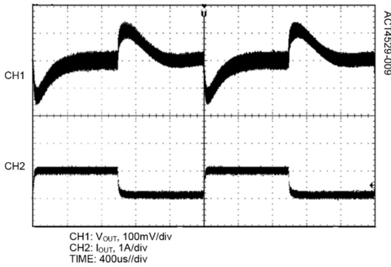
Load Transient (80mA-1A-80mA) V_{in}=12\text{V} , V_{out}=5\text{V}
