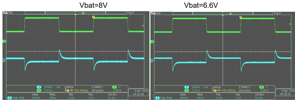
(Output2=1A-2.4A-1A load step Ouput1=1A)
