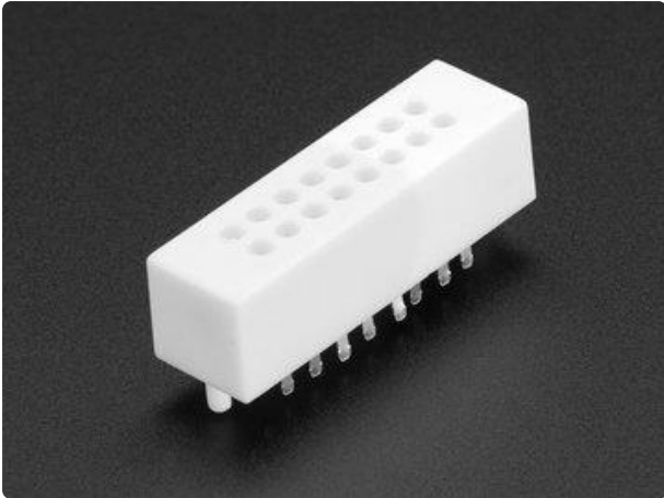
The 2x8 mini breadboard has 8 strips of 2-pin terminal strips ( http://adafru.it/2018 )
