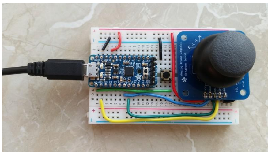
Trinket joystick by Mike Barela (https://adafru.it/rd5)
