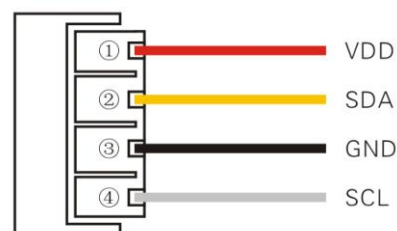
Figure 1: AM2315wiring diagram
